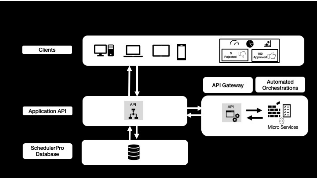
Figure 1. SchedulerPro architecture diagram
